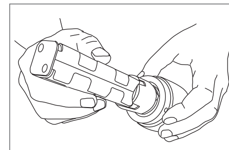
Drawing 9 - Insertion of the battery casing in the reflector-glass group (torch head)
