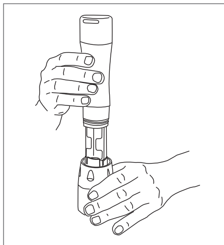
Drawing 12 - Insertion of the battery casing into the torch casing.
