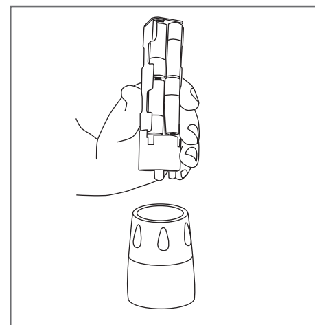
Drawing 4 - Removal of the battery casing
